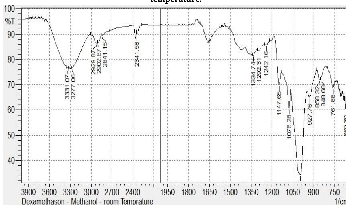
Figure 10. FTIR spectra of the crystals of dexamethasone obtained from methanolic solvent at room temperature.
